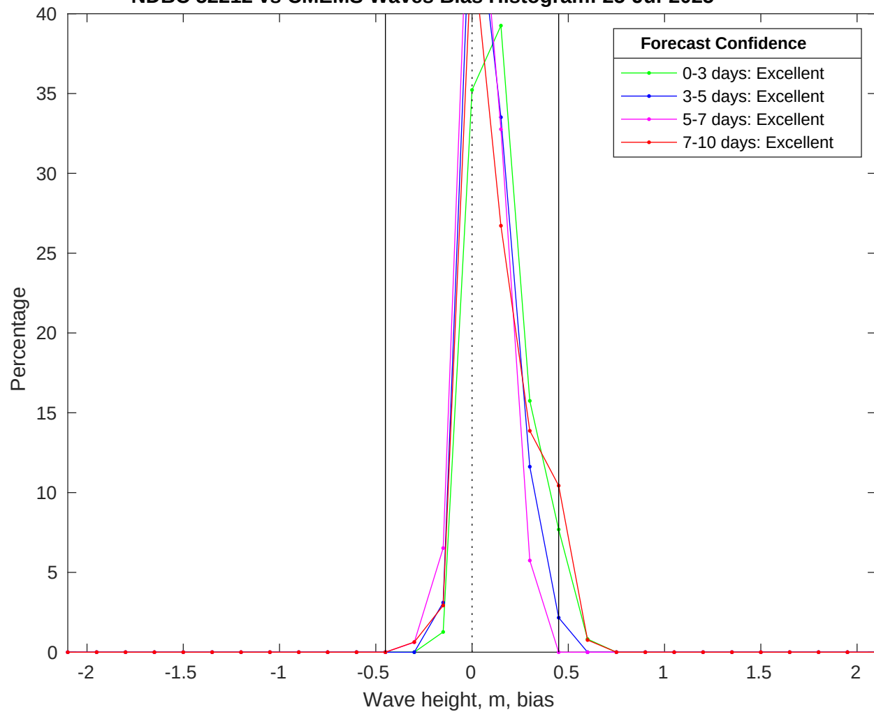
NDBC 52212 vs CMEMS Waves Bias Histogram: 25-Jul-2025
