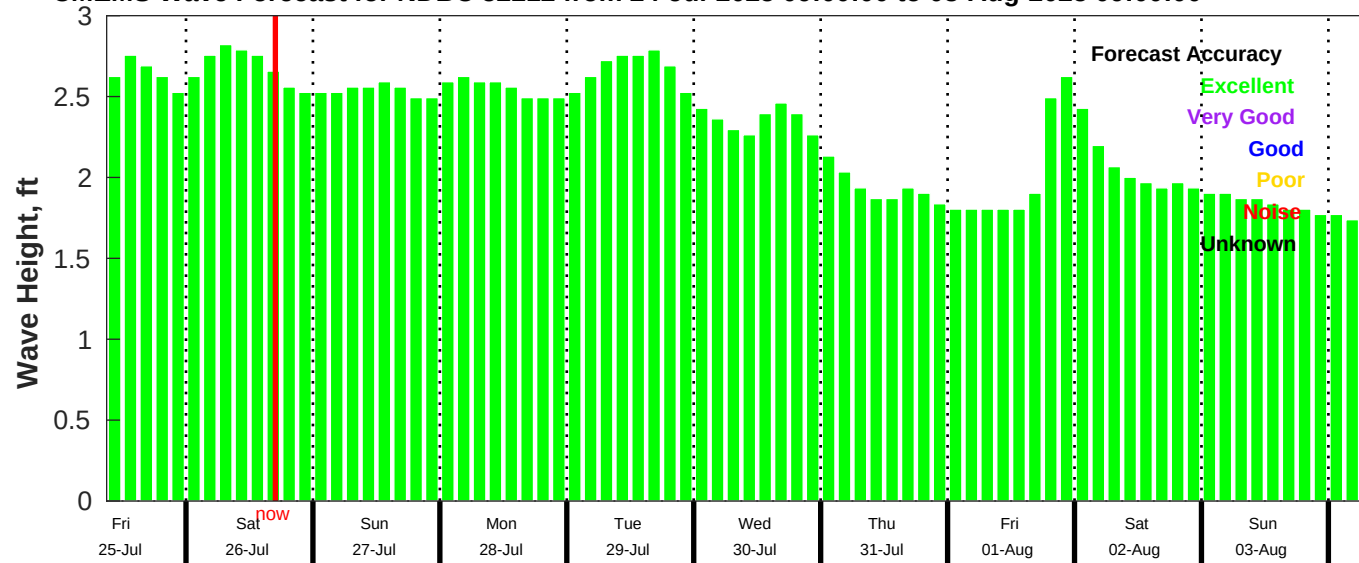
CMEMS Wave Forecast for NDBC 52212 from 24-Jul-2025 09:00:00 to 03-Aug-2025 09:00:00
