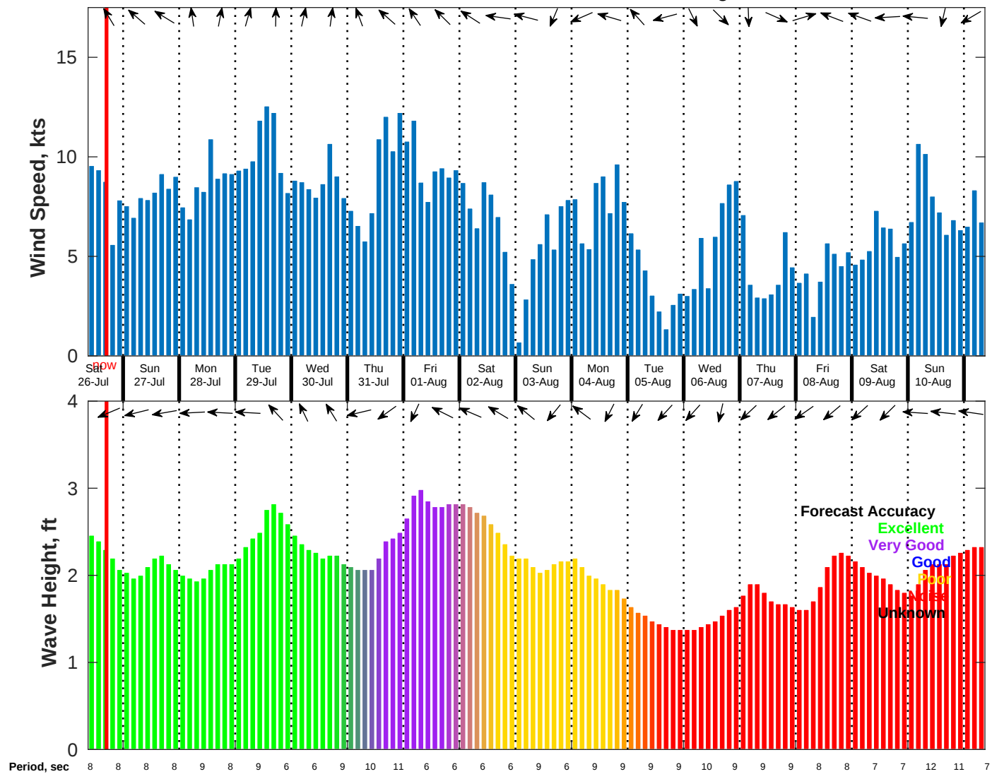
Wind & Wave Forecast for NDBC 52212 from 25-Jul-2025 09:00:00 to 10-Aug-2025 09:00:00
