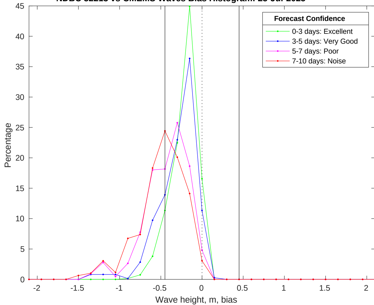
NDBC 52213 vs CMEMS Waves Bias Histogram: 25-Jul-2025
