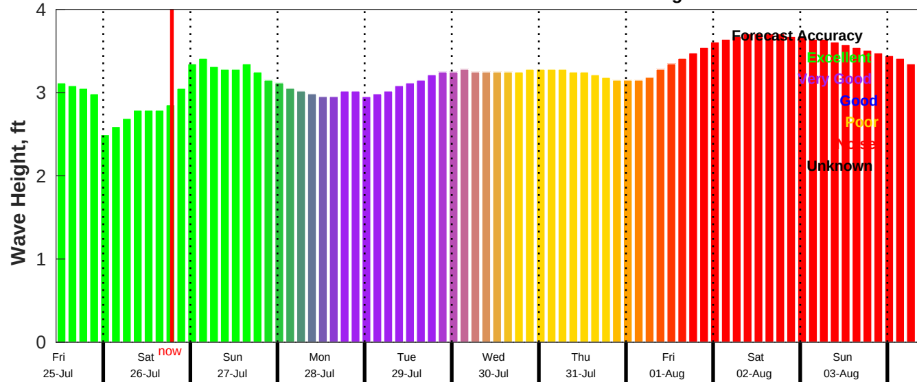
CMEMS Wave Forecast for NDBC 52213 from 24-Jul-2025 11:00:00 to 03-Aug-2025 11:00:00
