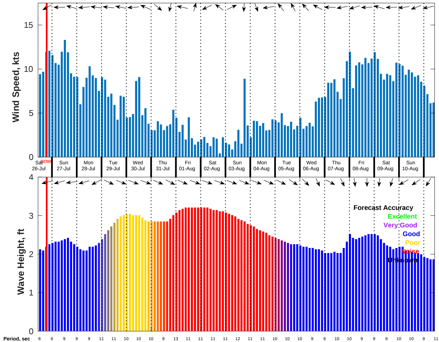
Wind & Wave Forecast for NDBC 52213 from 25-Jul-2025 11:00:00 to 10-Aug-2025 11:00:00
