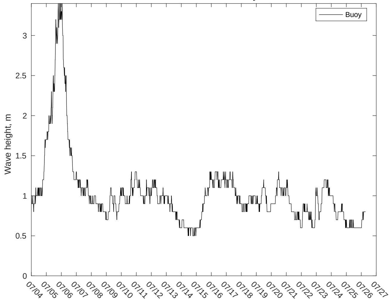
NDBC 41004 vs CMEMS Waves: 10 to 16 day forecast
