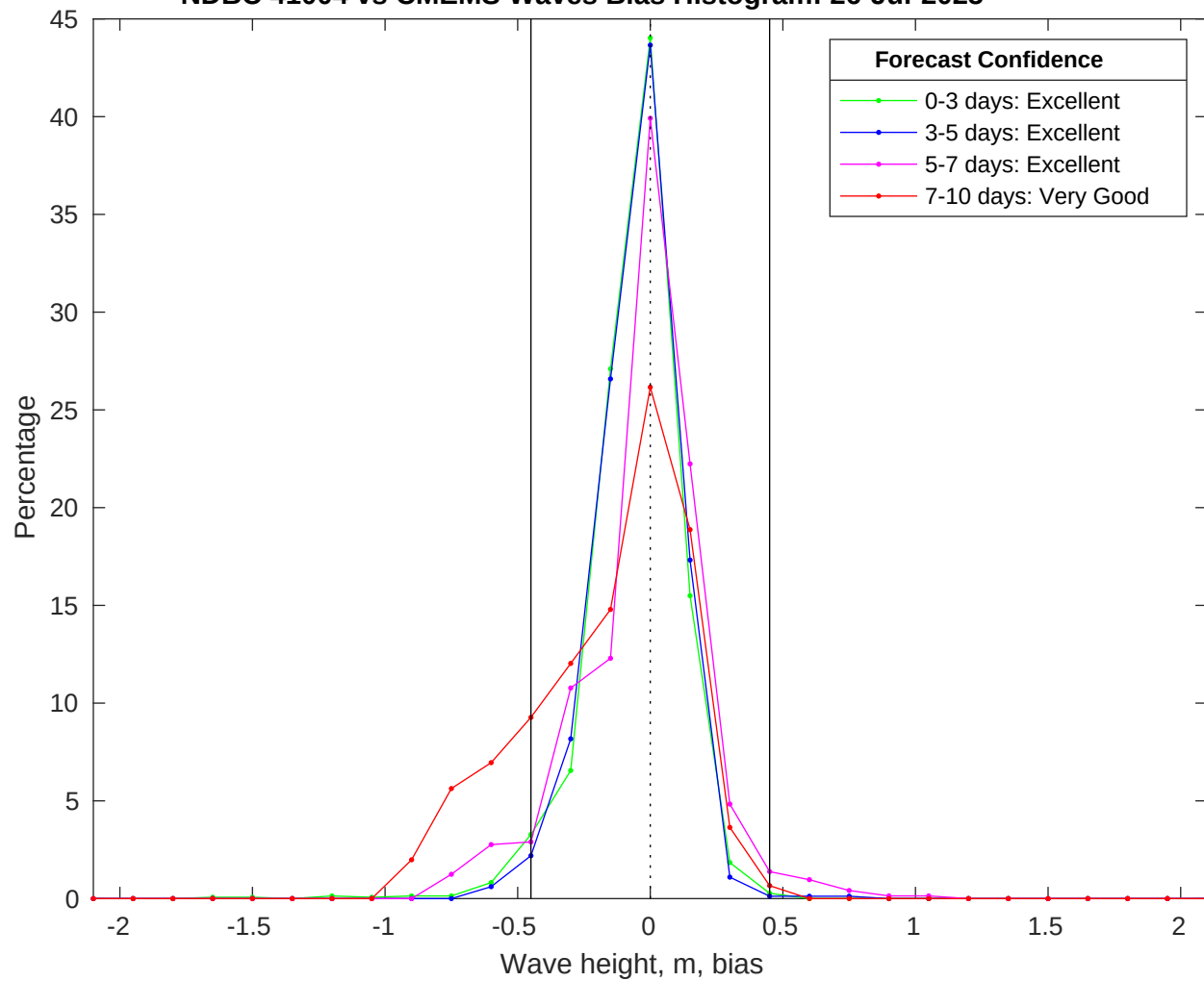
NDBC 41004 vs CMEMS Waves Bias Histogram: 26-Jul-2025
