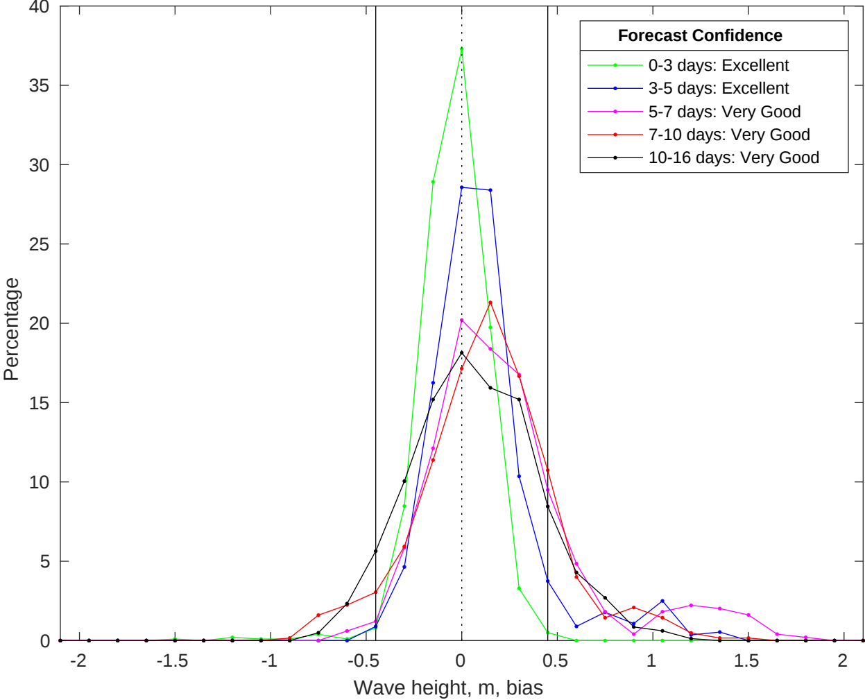
NDBC 41004 vs GFS Waves Bias Histogram: 26-Jul-2025
