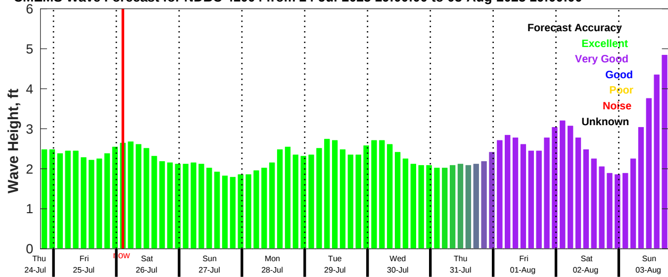
CMEMS Wave Forecast for NDBC 41004 from 24-Jul-2025 19:00:00 to 03-Aug-2025 19:00:00
