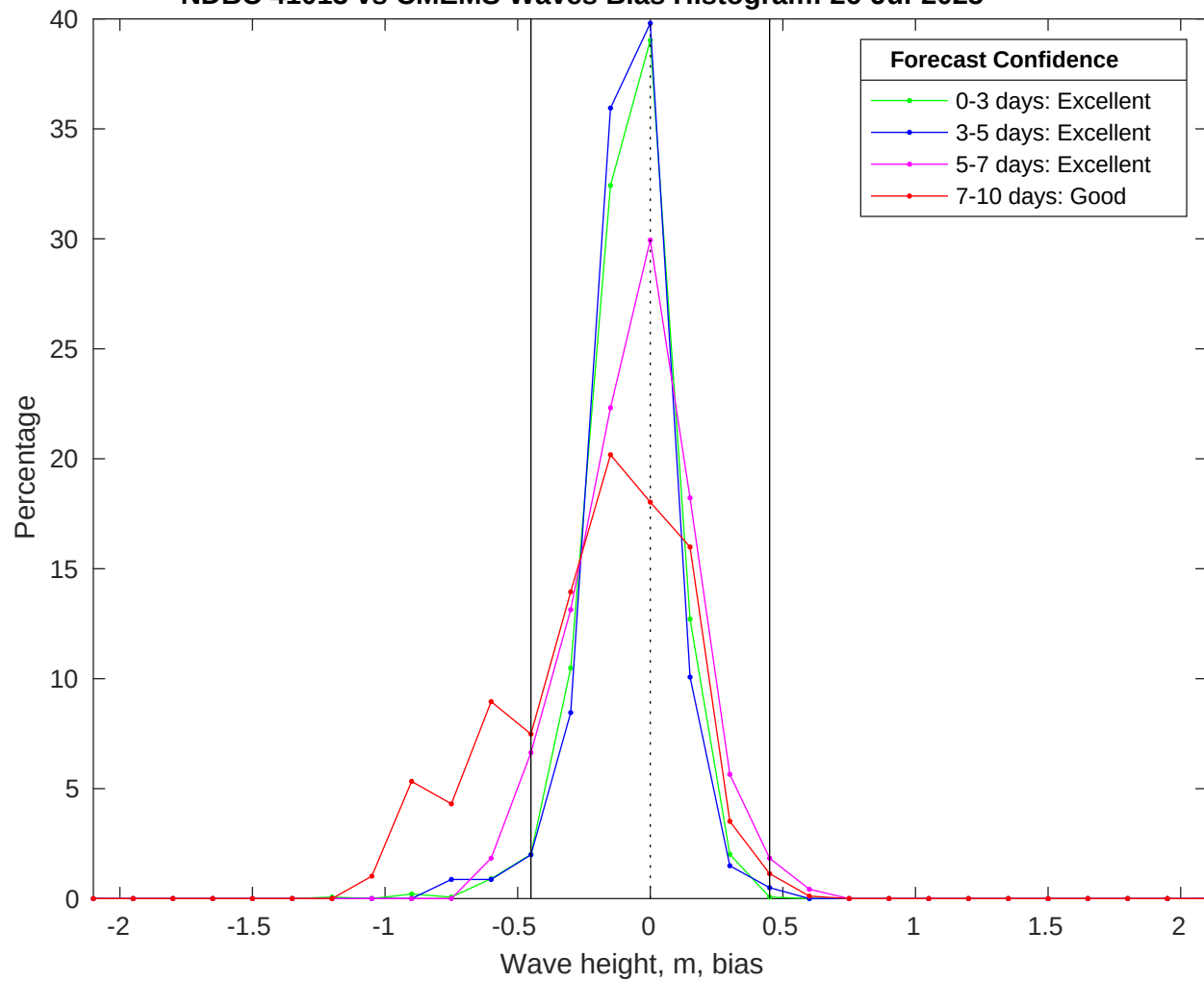
NDBC 41013 vs CMEMS Waves Bias Histogram: 26-Jul-2025
