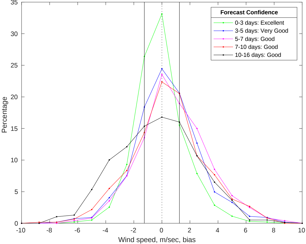
NDBC 41013 vs GFS Winds Bias Histogram: 26-Jul-2025
