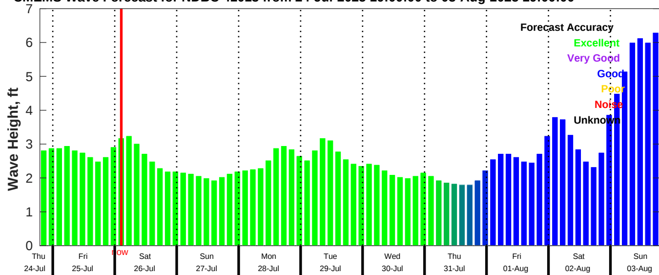
CMEMS Wave Forecast for NDBC 41013 from 24-Jul-2025 19:00:00 to 03-Aug-2025 19:00:00
