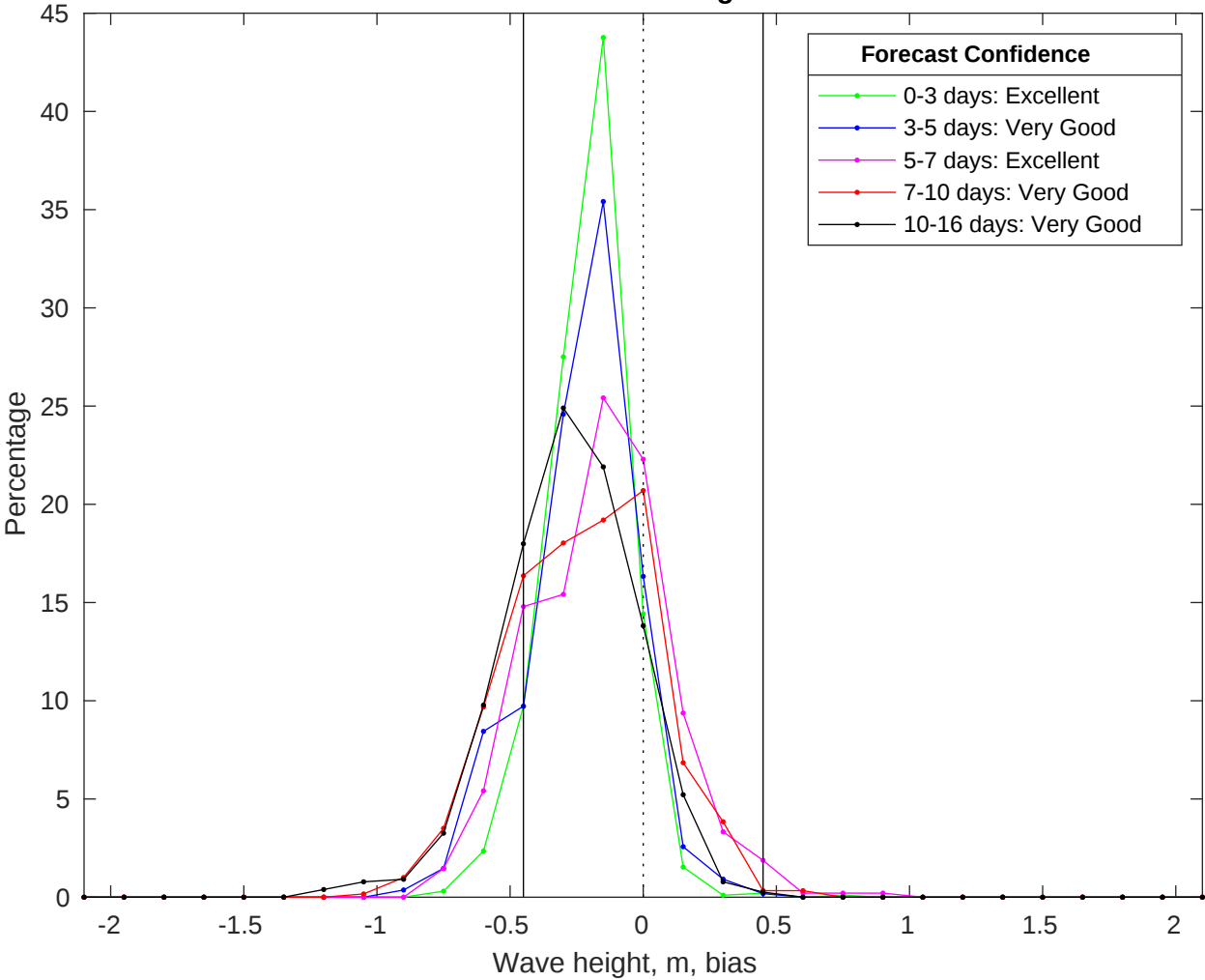
NDBC 41040 vs GFS Waves Bias Histogram: 26-Jul-2025
