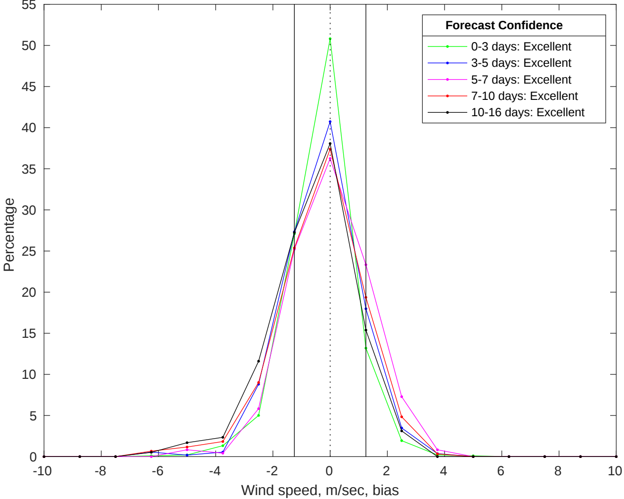
NDBC 41040 vs GFS Winds Bias Histogram: 26-Jul-2025
