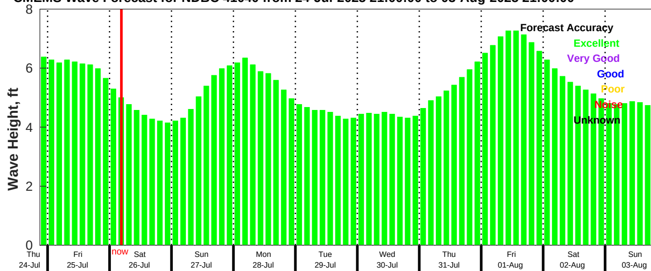
CMEMS Wave Forecast for NDBC 41040 from 24-Jul-2025 21:00:00 to 03-Aug-2025 21:00:00
