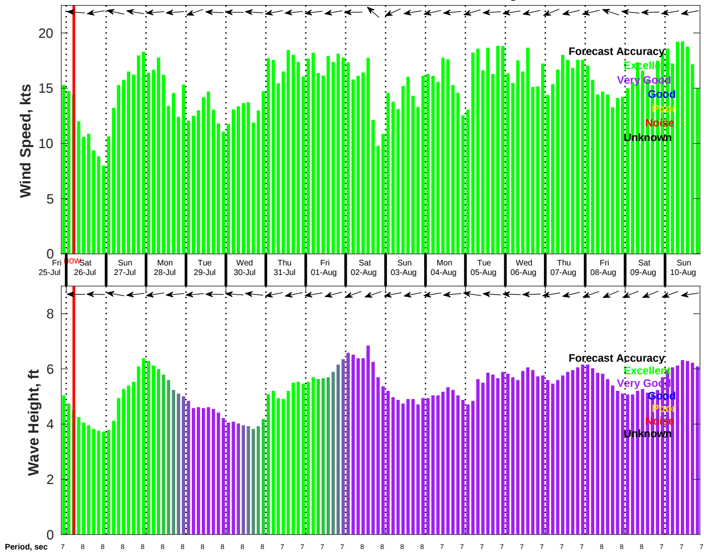
Wind & Wave Forecast for NDBC 41040 from 25-Jul-2025 21:00:00 to 10-Aug-2025 21:00:00
