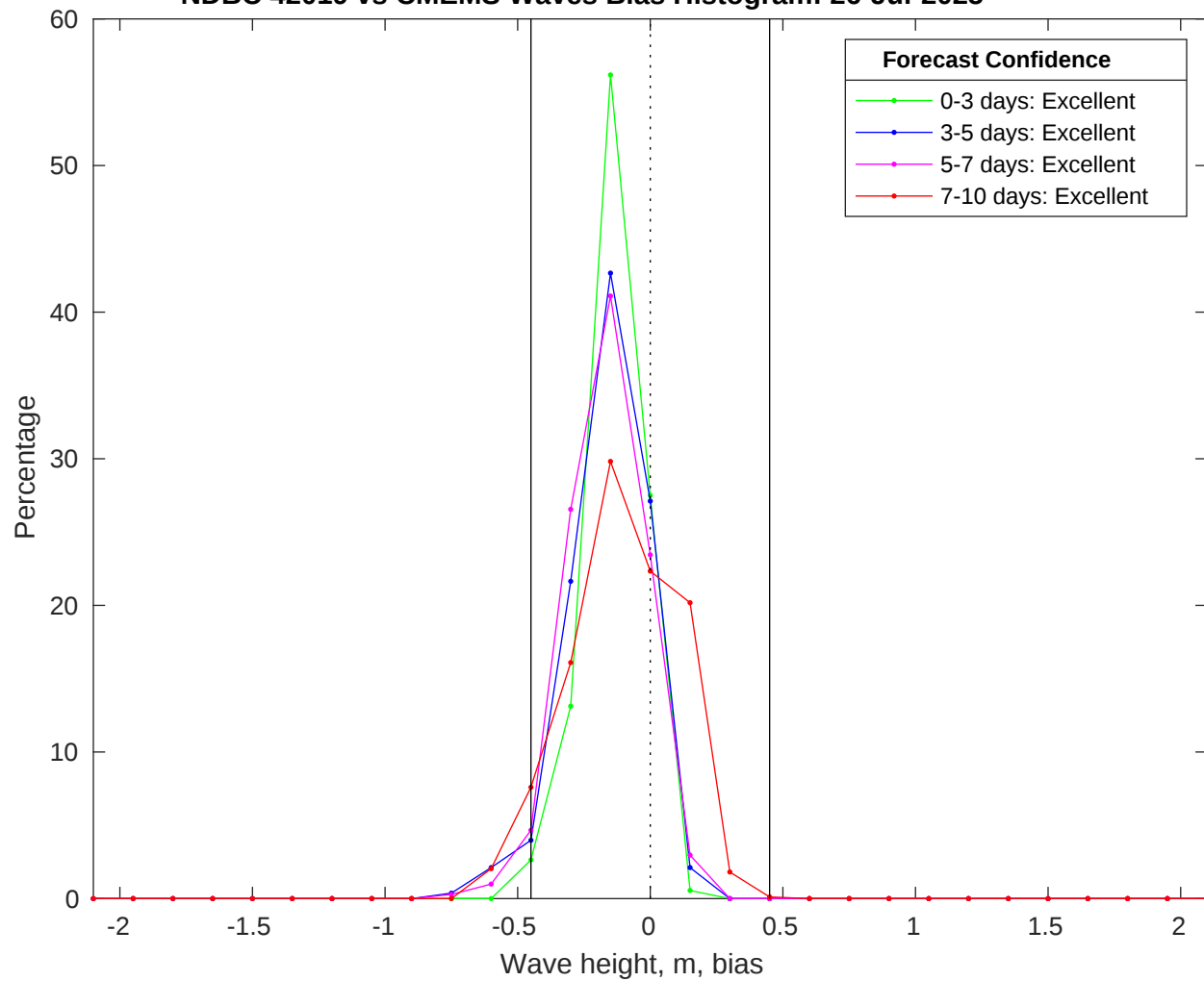
NDBC 42019 vs CMEMS Waves Bias Histogram: 26-Jul-2025
