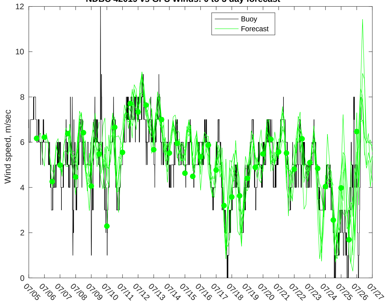
NDBC 42019 vs GFS Winds: 0 to 3 day forecast
