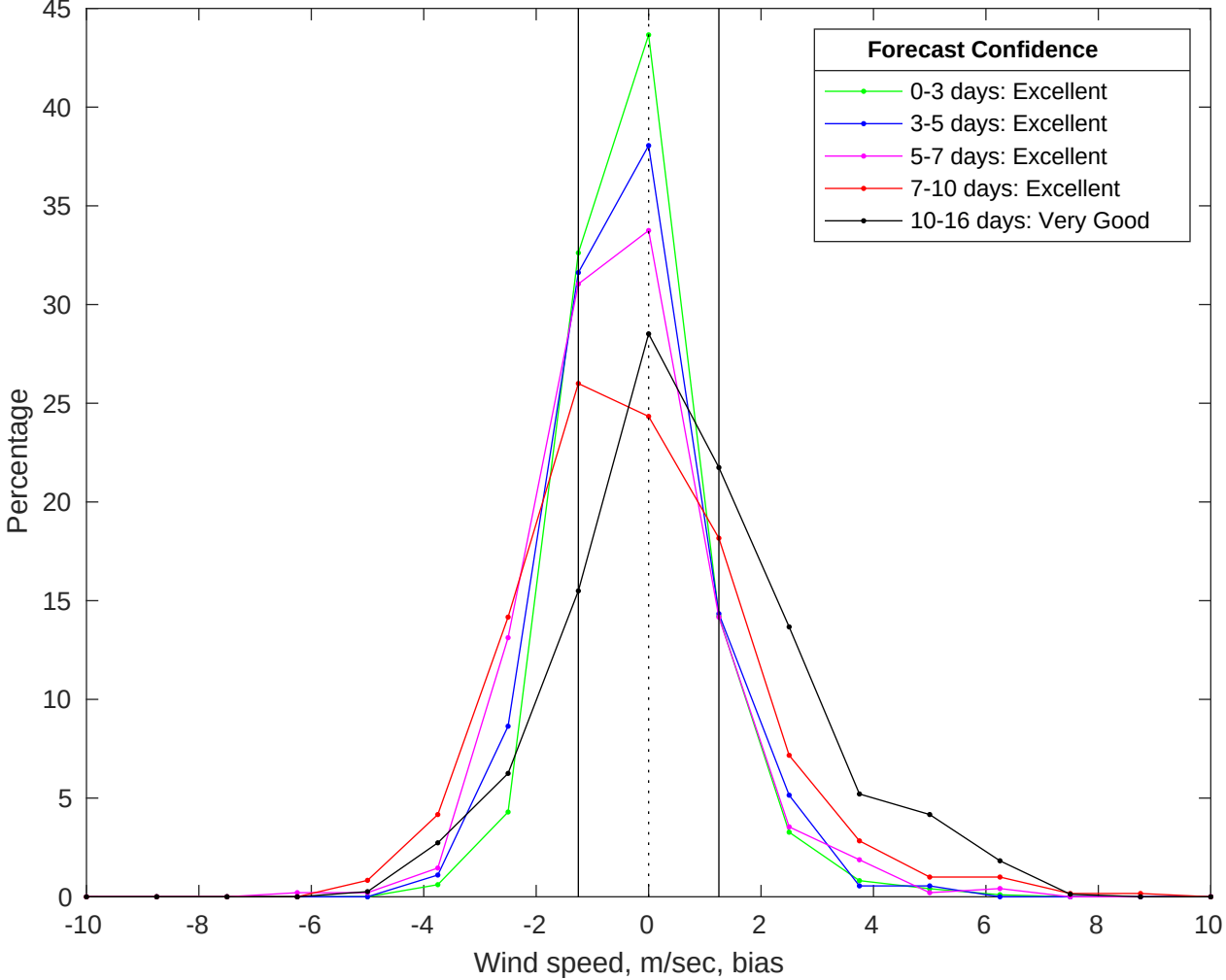
NDBC 42019 vs GFS Winds Bias Histogram: 26-Jul-2025
