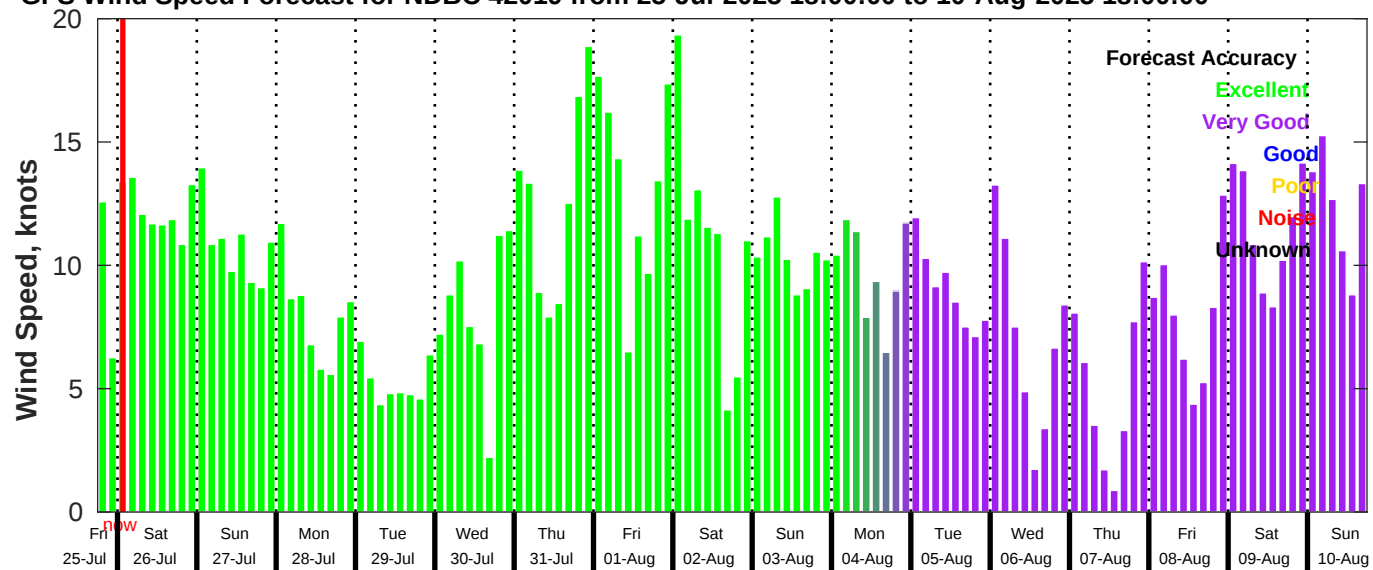
GFS Wind Speed Forecast for NDBC 42019 from 25-Jul-2025 18:00:00 to 10-Aug-2025 18:00:00
