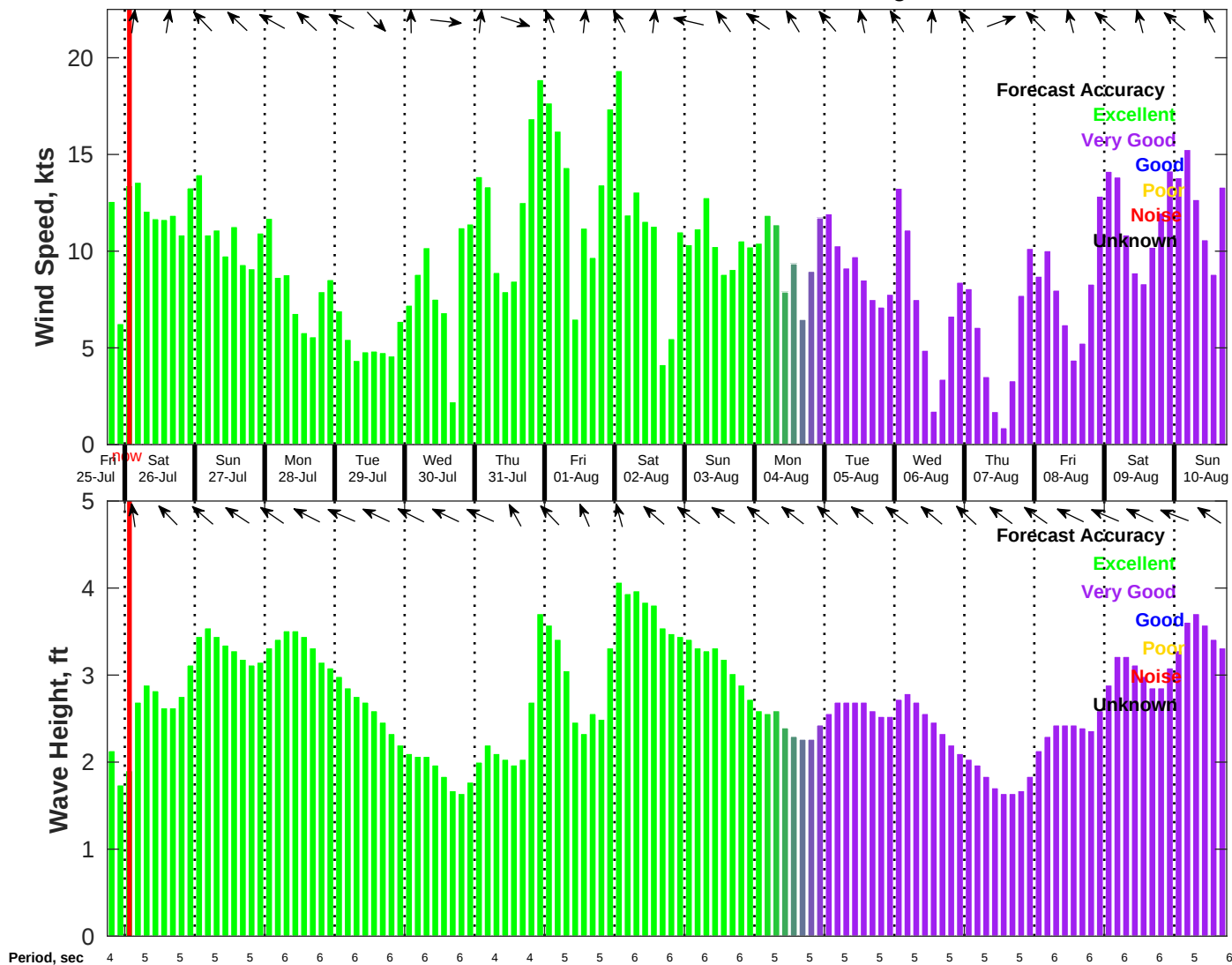
Wind & Wave Forecast for NDBC 42019 from 25-Jul-2025 18:00:00 to 10-Aug-2025 18:00:00
