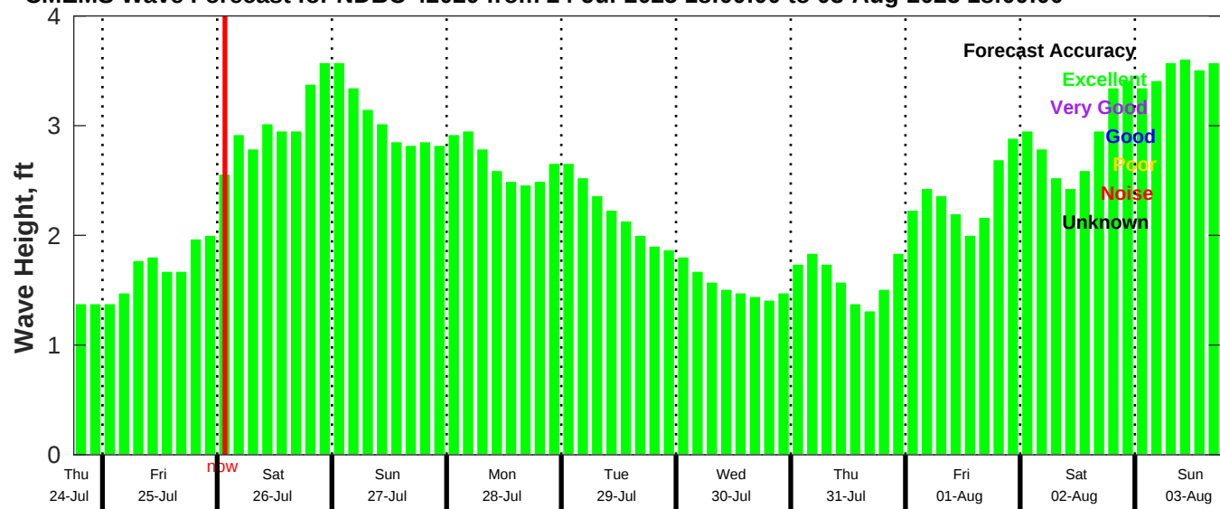
CMEMS Wave Forecast for NDBC 42020 from 24-Jul-2025 18:00:00 to 03-Aug-2025 18:00:00
