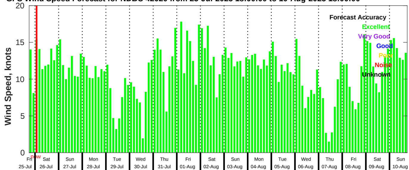
GFS Wind Speed Forecast for NDBC 42020 from 25-Jul-2025 18:00:00 to 10-Aug-2025 18:00:00
