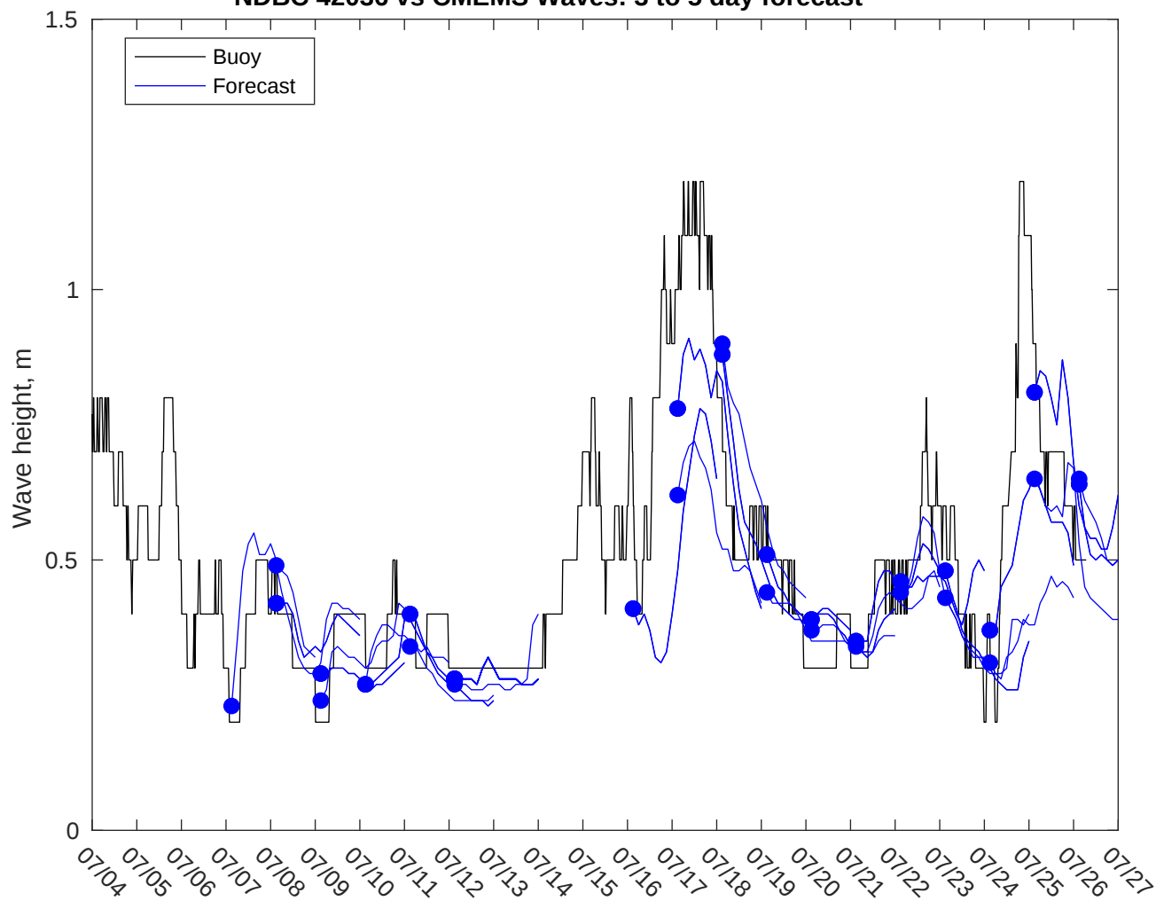
NDBC 42036 vs CMEMS Waves: 3 to 5 day forecast
