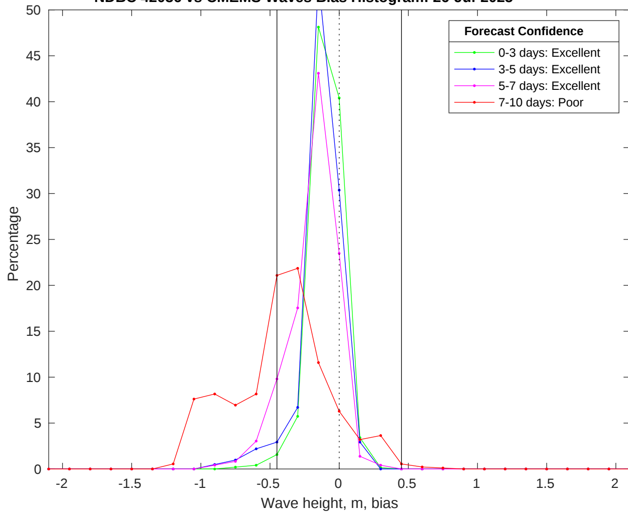
NDBC 42036 vs CMEMS Waves Bias Histogram: 26-Jul-2025
