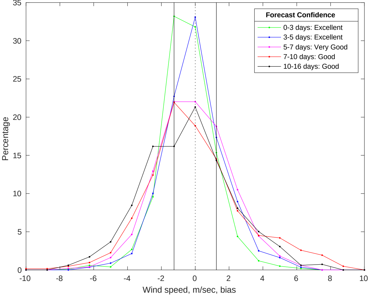
NDBC 42036 vs GFS Winds Bias Histogram: 26-Jul-2025
