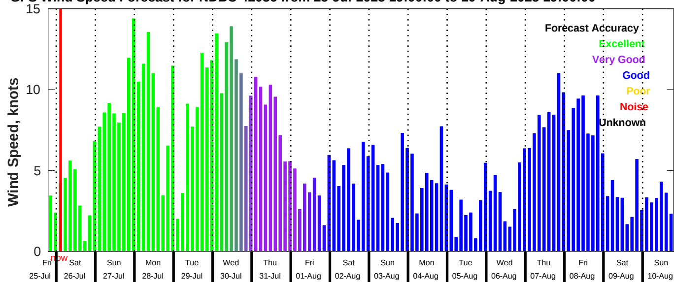
GFS Wind Speed Forecast for NDBC 42036 from 25-Jul-2025 19:00:00 to 10-Aug-2025 19:00:00
