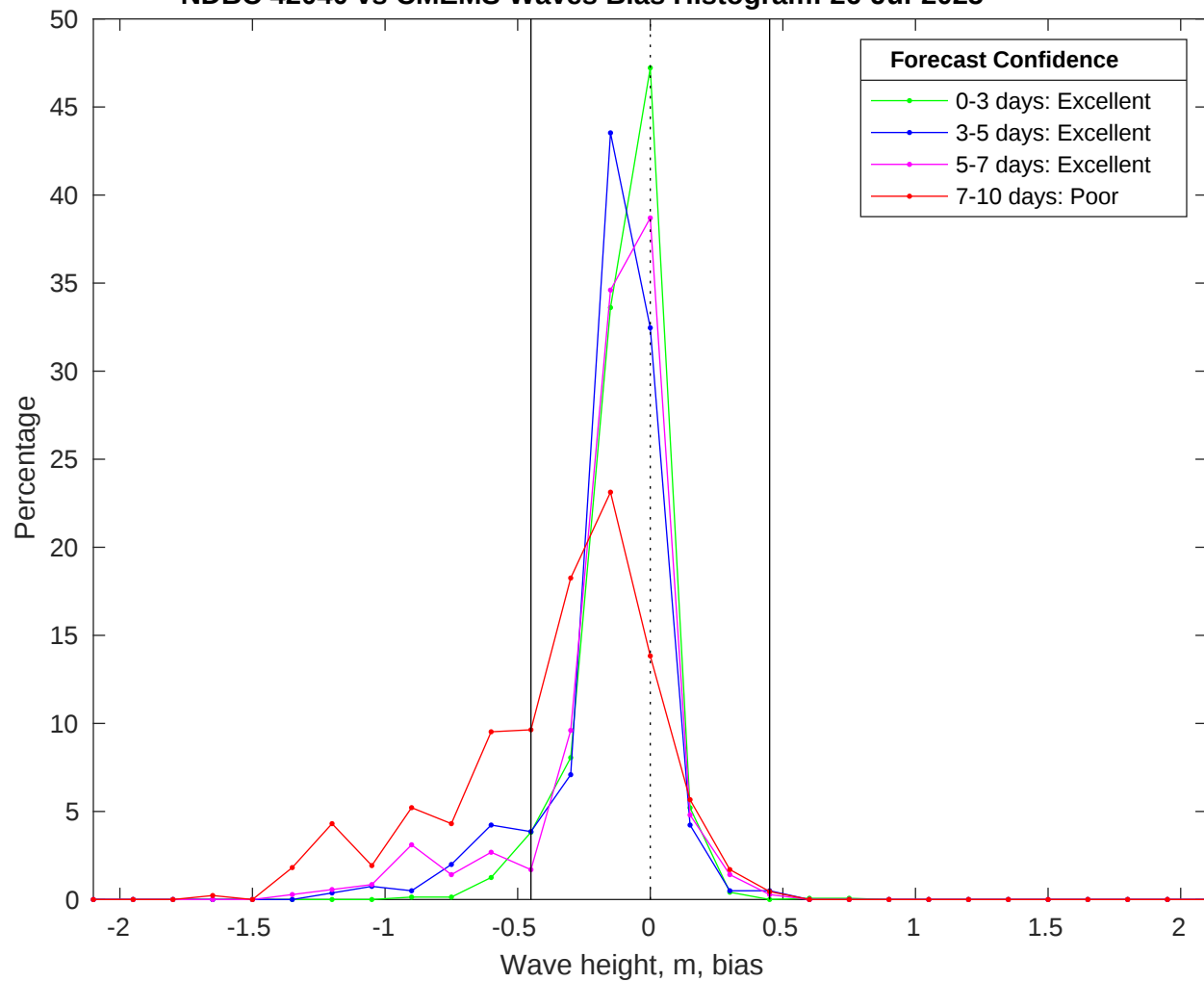
NDBC 42040 vs CMEMS Waves Bias Histogram: 26-Jul-2025
