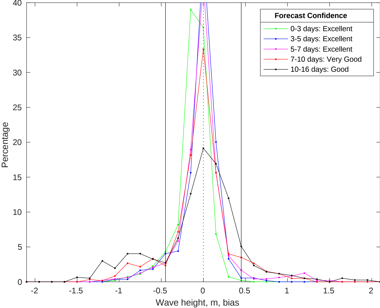
NDBC 42040 vs GFS Waves Bias Histogram: 26-Jul-2025
