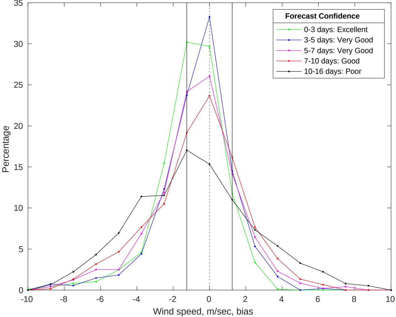
NDBC 42040 vs GFS Winds Bias Histogram: 26-Jul-2025
