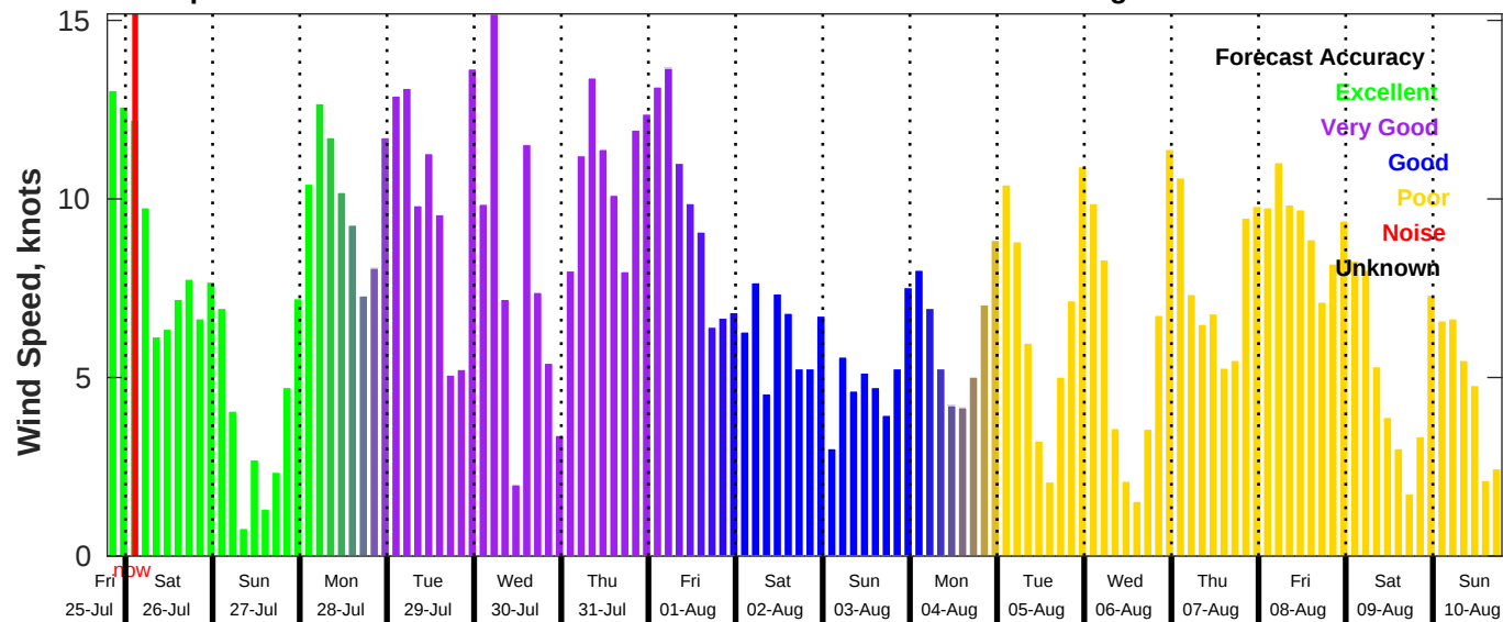
GFS Wind Speed Forecast for NDBC 42040 from 25-Jul-2025 19:00:00 to 10-Aug-2025 19:00:00
