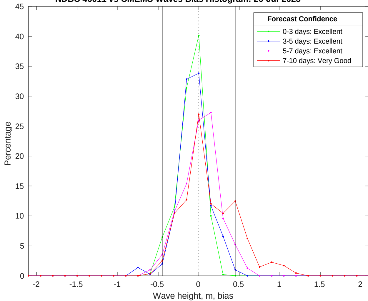
NDBC 46011 vs CMEMS Waves Bias Histogram: 26-Jul-2025
