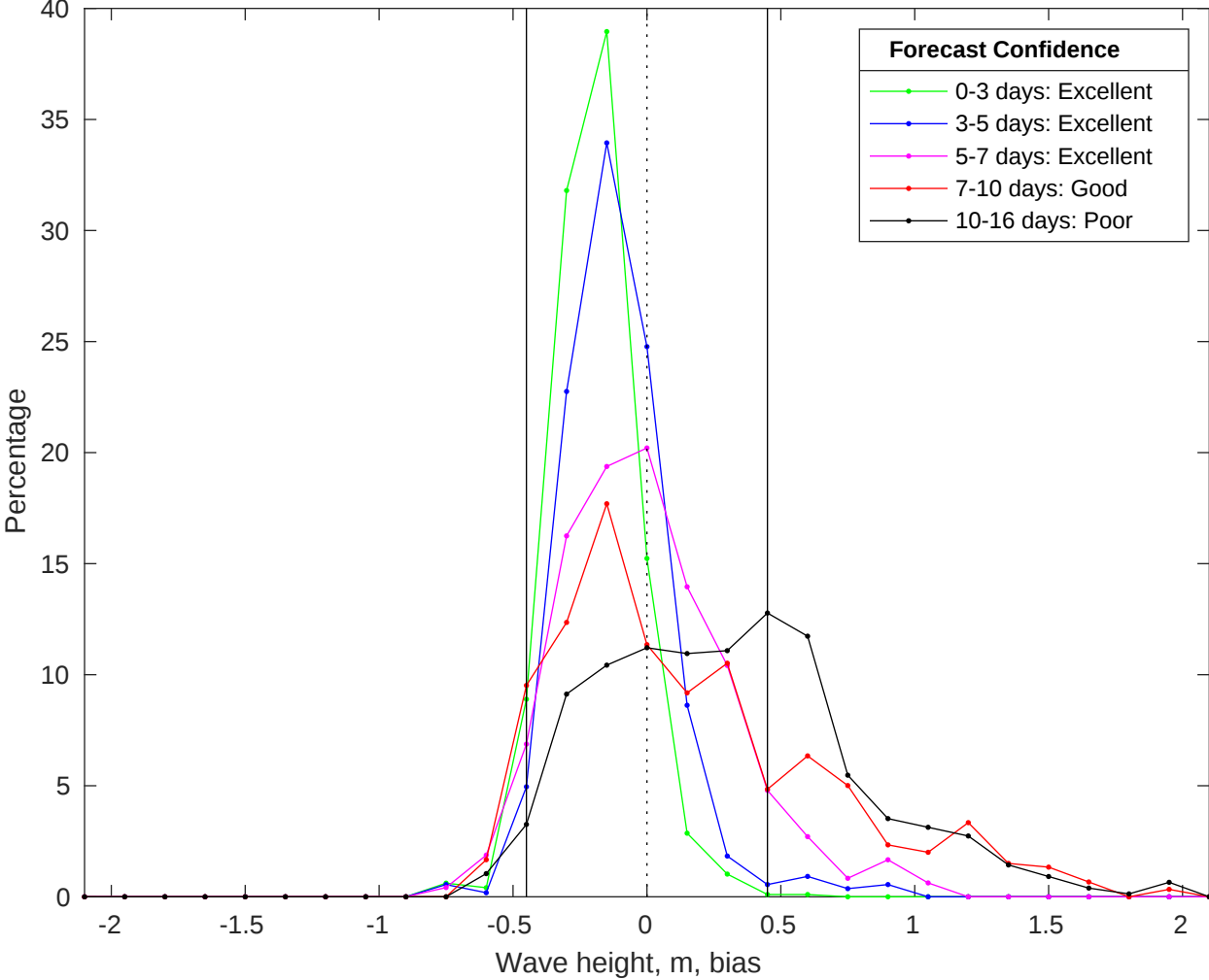
NDBC 46011 vs GFS Waves Bias Histogram: 26-Jul-2025
