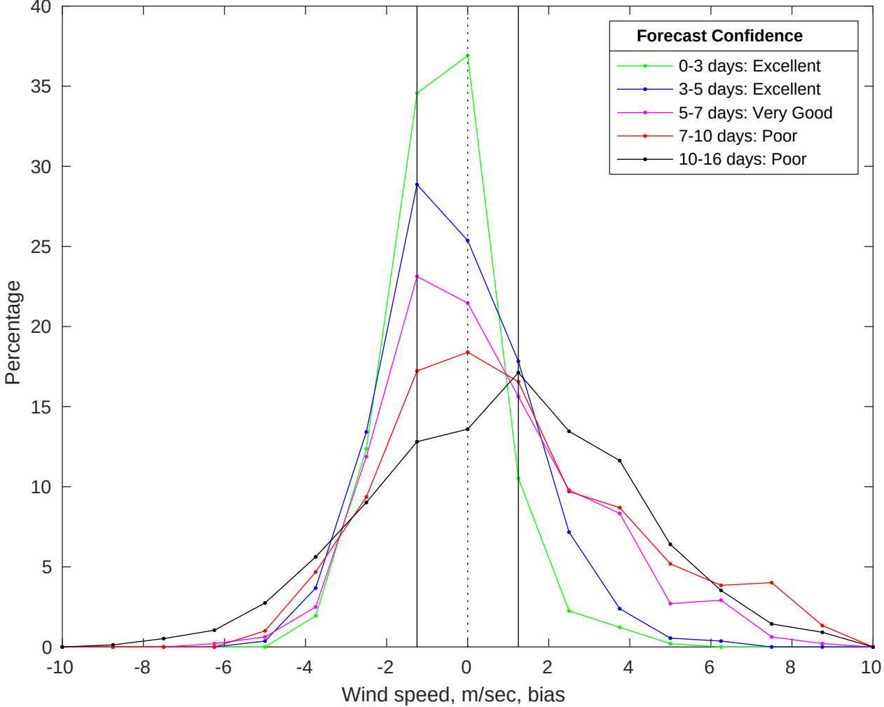
NDBC 46011 vs GFS Winds Bias Histogram: 26-Jul-2025
