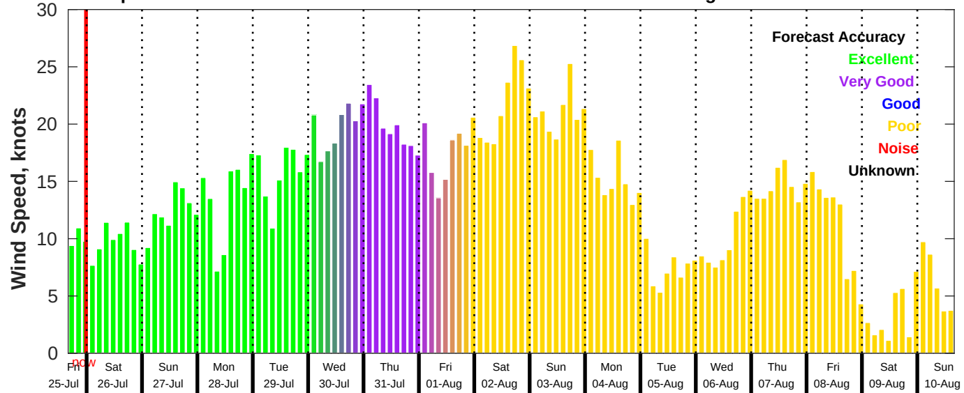
GFS Wind Speed Forecast for NDBC 46011 from 25-Jul-2025 16:00:00 to 10-Aug-2025 16:00:00
