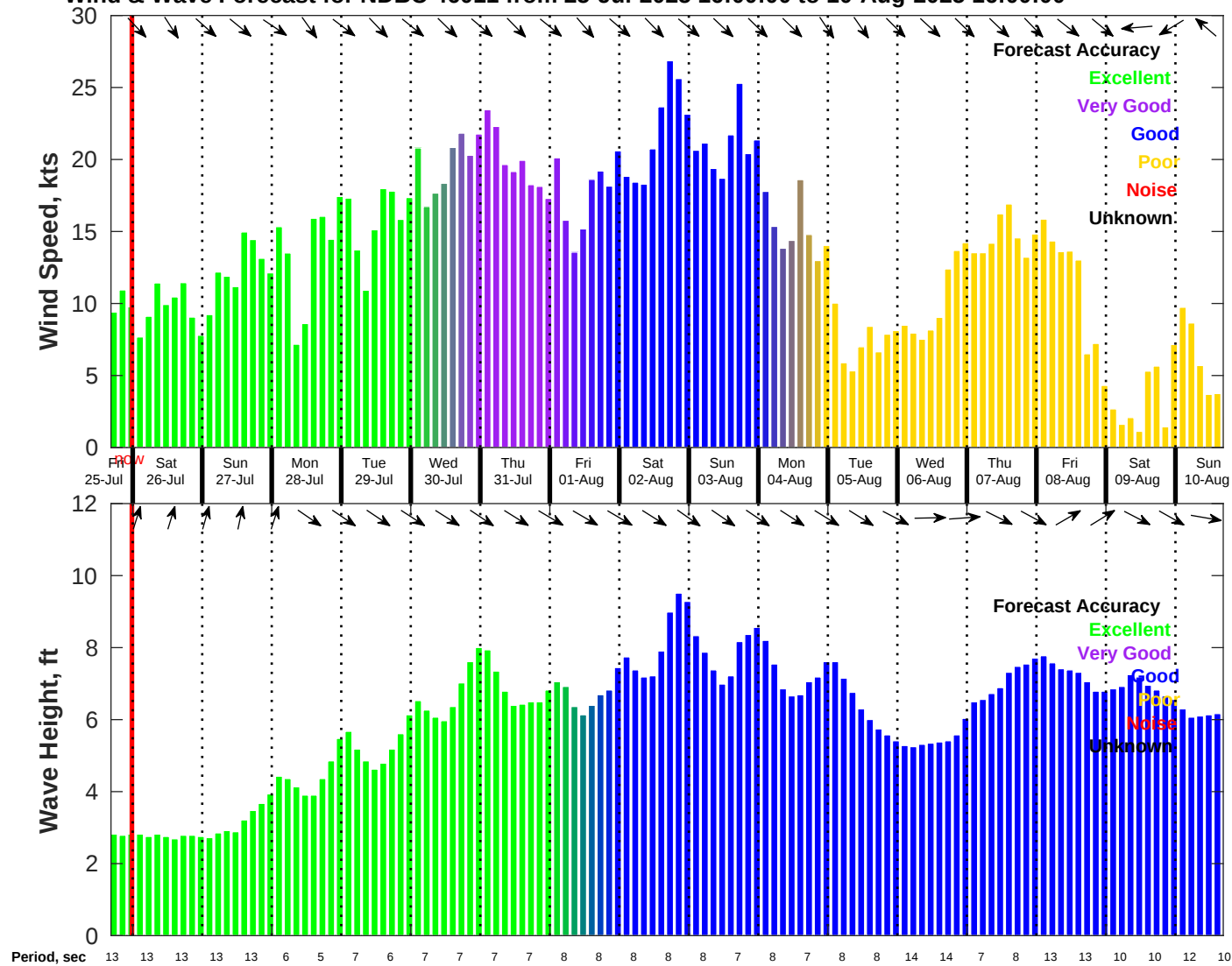
Wind & Wave Forecast for NDBC 46011 from 25-Jul-2025 16:00:00 to 10-Aug-2025 16:00:00
