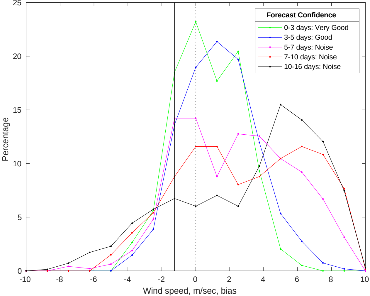
NDBC 46028 vs GFS Winds Bias Histogram: 26-Jul-2025
