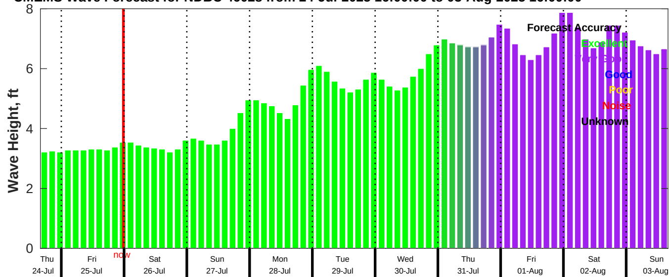
CMEMS Wave Forecast for NDBC 46028 from 24-Jul-2025 16:00:00 to 03-Aug-2025 16:00:00
