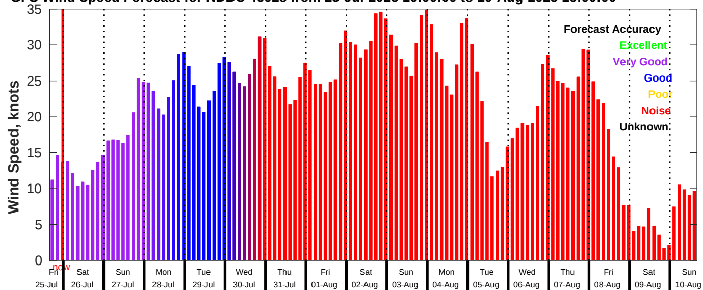
GFS Wind Speed Forecast for NDBC 46028 from 25-Jul-2025 16:00:00 to 10-Aug-2025 16:00:00
