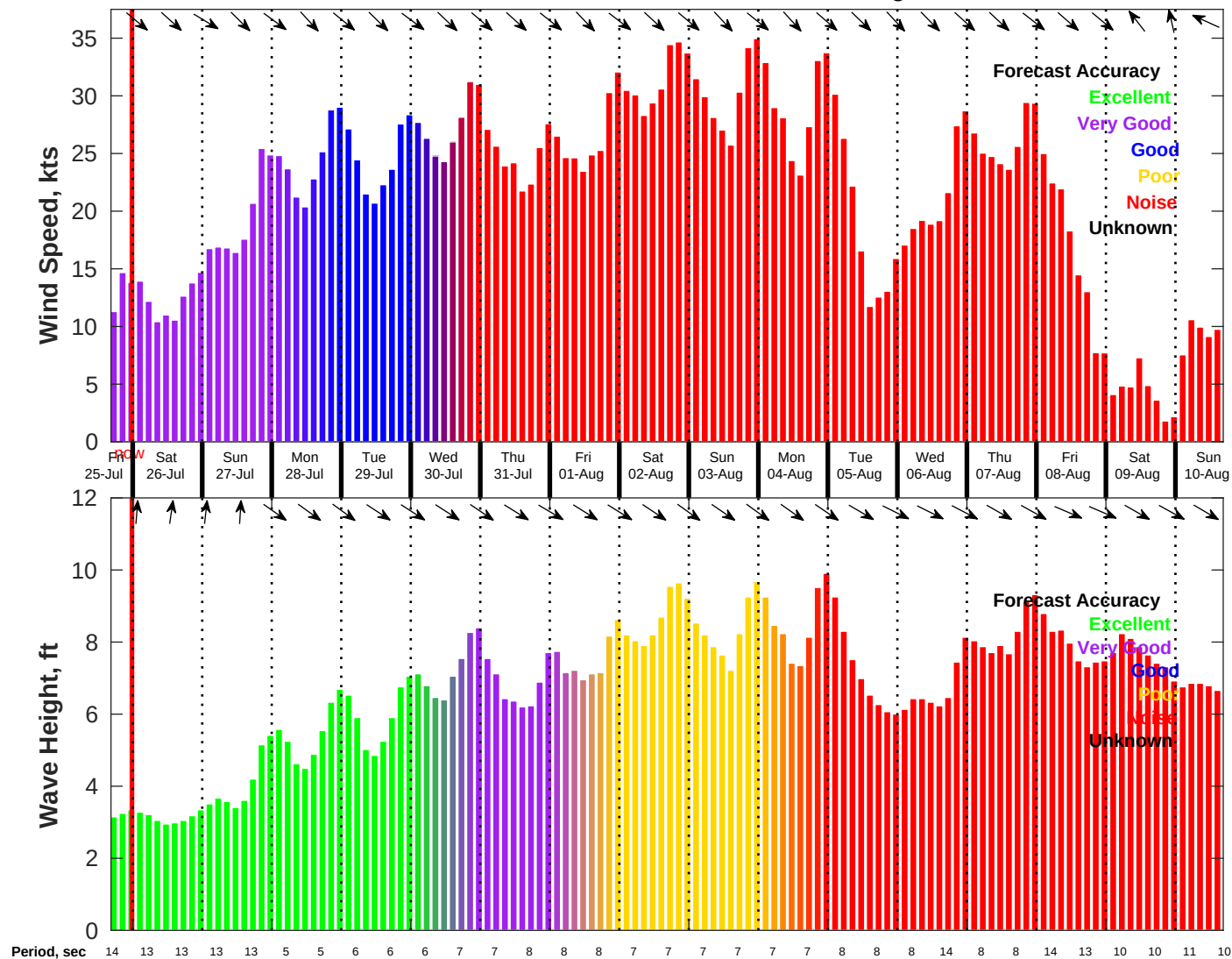
Wind & Wave Forecast for NDBC 46028 from 25-Jul-2025 16:00:00 to 10-Aug-2025 16:00:00
