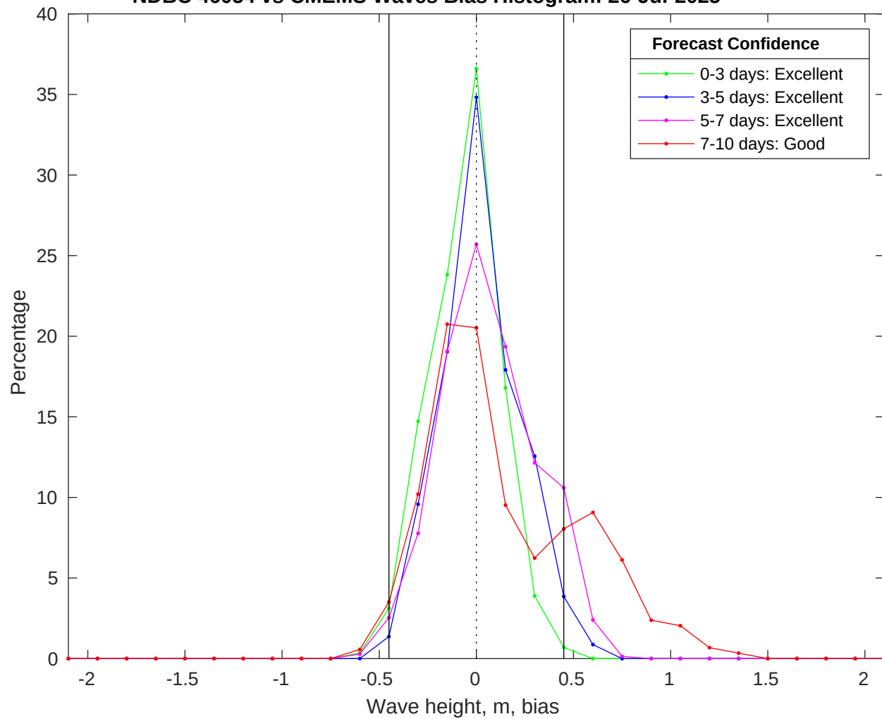
NDBC 46054 vs CMEMS Waves Bias Histogram: 26-Jul-2025
