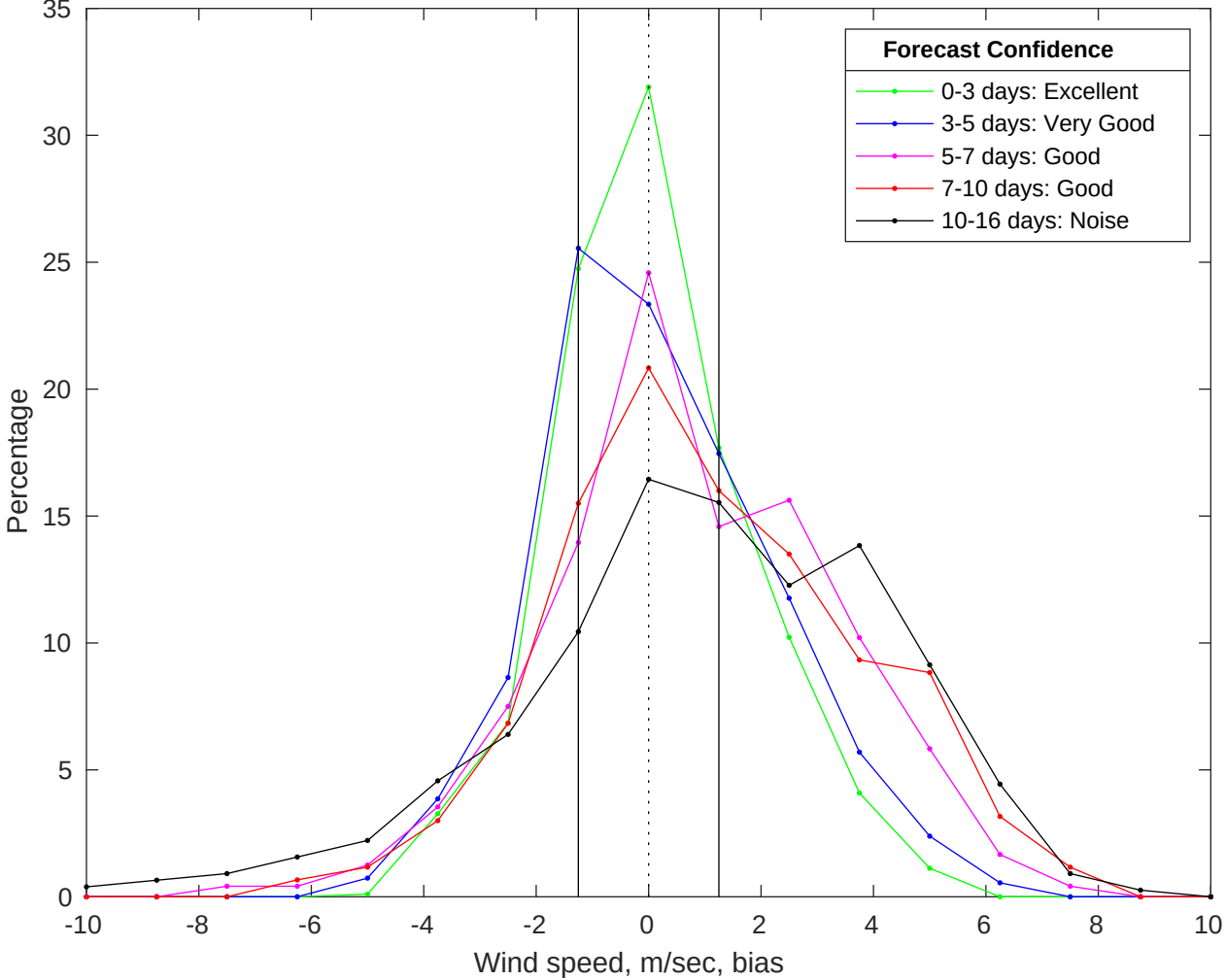
NDBC 46054 vs GFS Winds Bias Histogram: 26-Jul-2025
