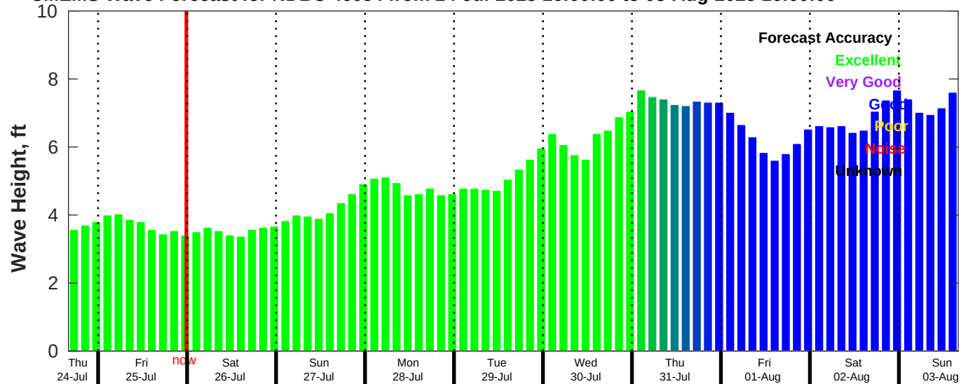
CMEMS Wave Forecast for NDBC 46054 from 24-Jul-2025 16:00:00 to 03-Aug-2025 16:00:00
