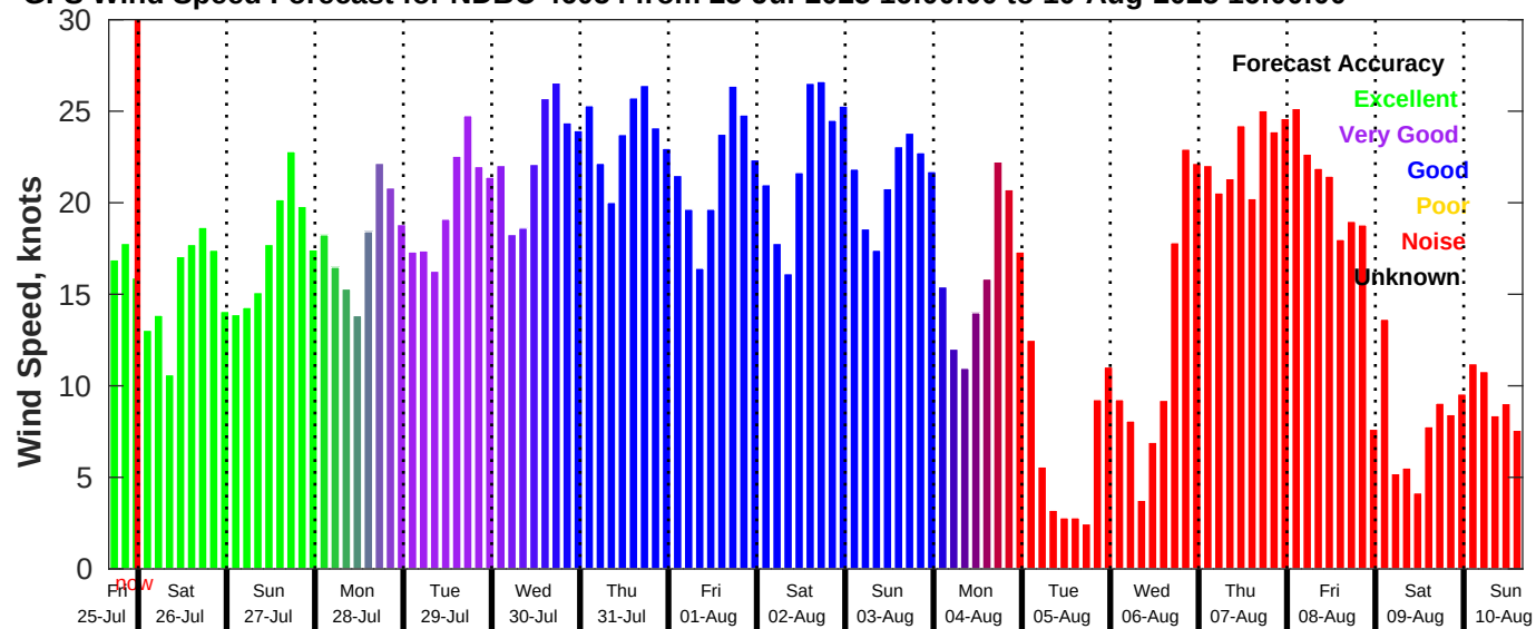
GFS Wind Speed Forecast for NDBC 46054 from 25-Jul-2025 16:00:00 to 10-Aug-2025 16:00:00
