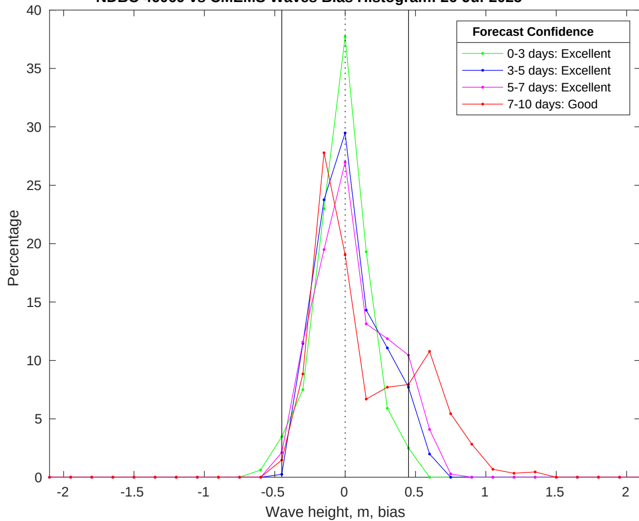
NDBC 46069 vs CMEMS Waves Bias Histogram: 26-Jul-2025
