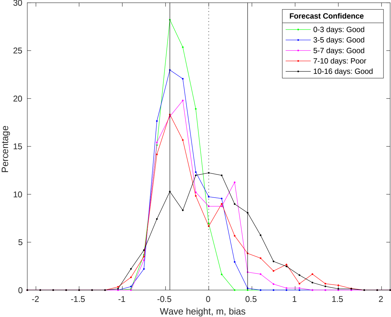
NDBC 46069 vs GFS Waves Bias Histogram: 26-Jul-2025
