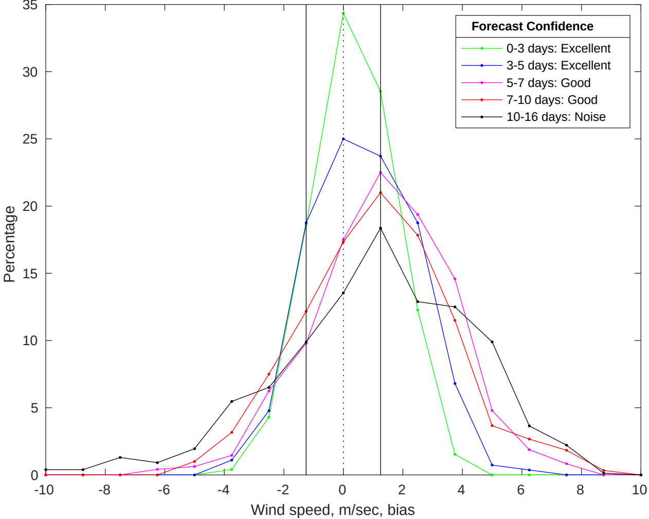
NDBC 46069 vs GFS Winds Bias Histogram: 26-Jul-2025
