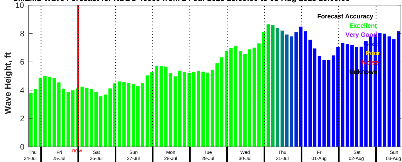
CMEMS Wave Forecast for NDBC 46069 from 24-Jul-2025 16:00:00 to 03-Aug-2025 16:00:00
