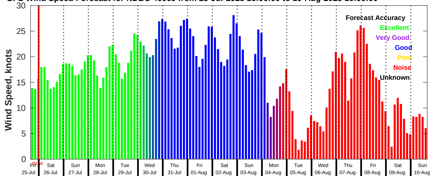
GFS Wind Speed Forecast for NDBC 46069 from 25-Jul-2025 16:00:00 to 10-Aug-2025 16:00:00
